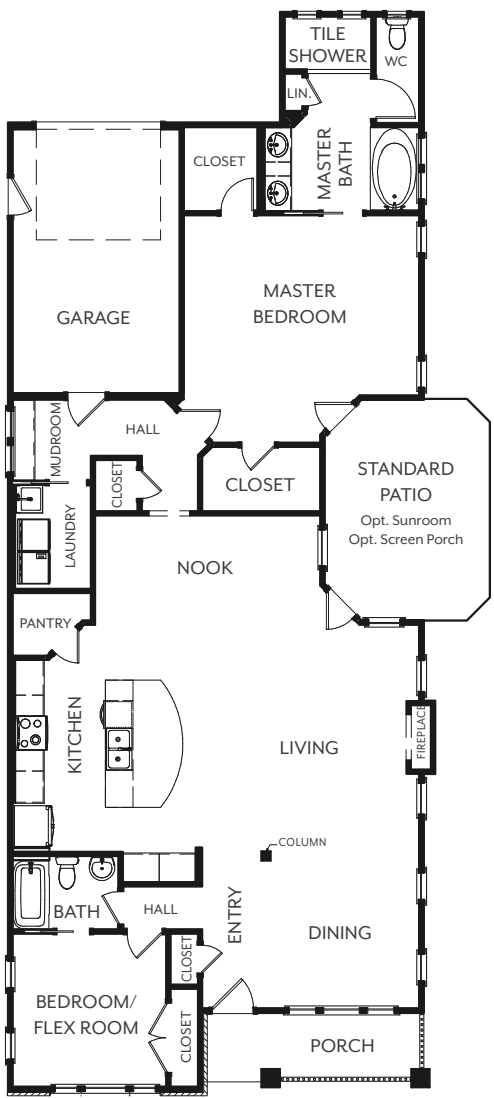
First Floor with 1-Car Garage Option
